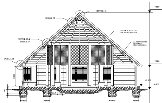
READING ROOM SECTION
